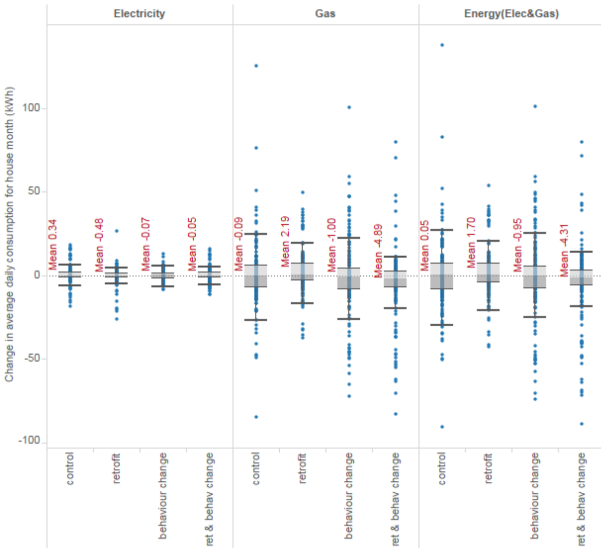
Figure 2. Change in average daily energy consumption for house months (using data from monitoring equipment). Each dot represents one house month; box shows median and interquartile range; whiskers show 1.5 times interquartile.
